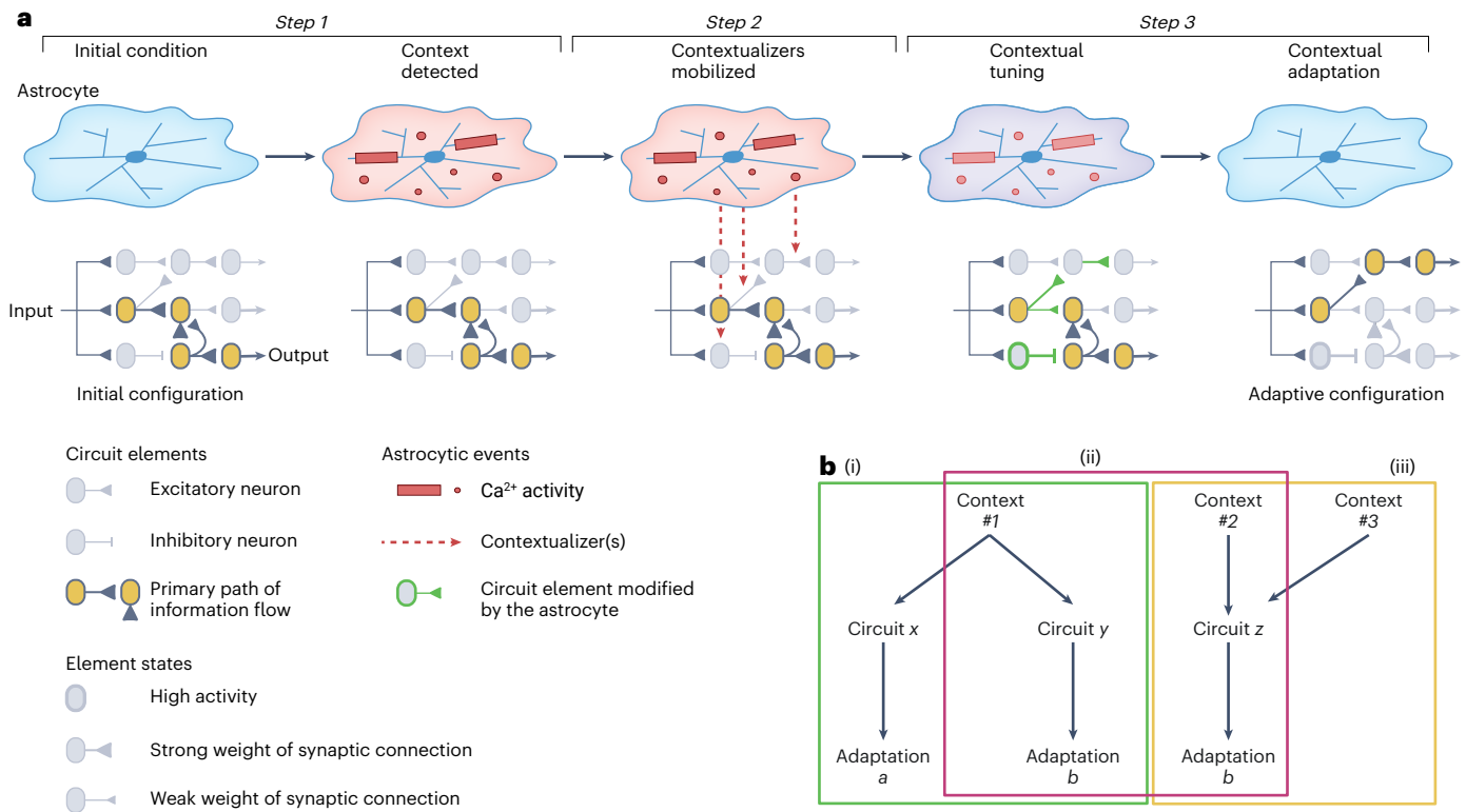
Fig. 2 | Astrocytes reconfigure circuits in a context-dependent fashion. a , Stepwise illustration of the contextual guidance proposal, showing an individual astrocyte and embedded neuronal circuit over time. The astrocyte responds to the emergence of a context (shown as Ca 2+ transients). This leads to the mobilization of circuit-modifying contextualizer(s), which act on select elements (here presynaptic strength as in ref. 77 and interneuron firing as in ref. 48). These
