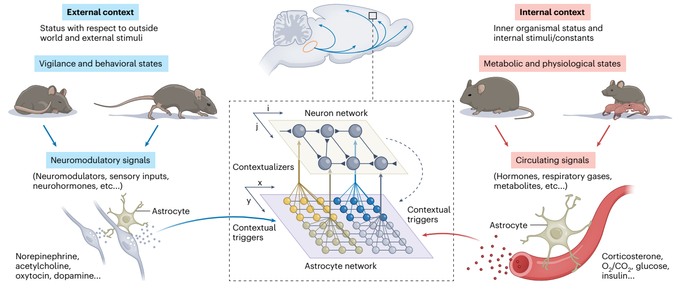
Fig. 1 | Astrocyte networks are cued by contextual signals to guide neural circuits. In contextual guidance, neuronal networks operate rapid point-to-point transfer and integration of information, while astrocytic networks transduce slower modulatory information over large spatial scales. In this proposed framework, astrocytes act as the primary receiver of slow contextual signals, such as neuromodulators, sensory inputs and neurohormones, that carry information about the status of the animal with respect to the outside world (left). Owing to their interactions with blood vessels, they are also the first responders to circulating signals, such as corticosterone, glucose and
